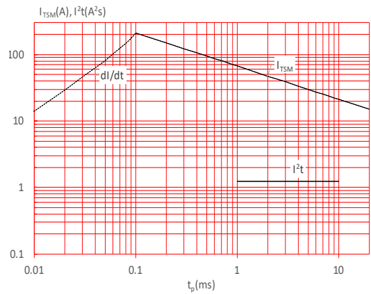
FIG.6: Non-repetitive surge peak on-state current for a sinusoidal pulse with width t_p < 20\text{ms} , and corresponding value of I^2t ( di/dt < 60\text{A}/\mu\text{s} )
